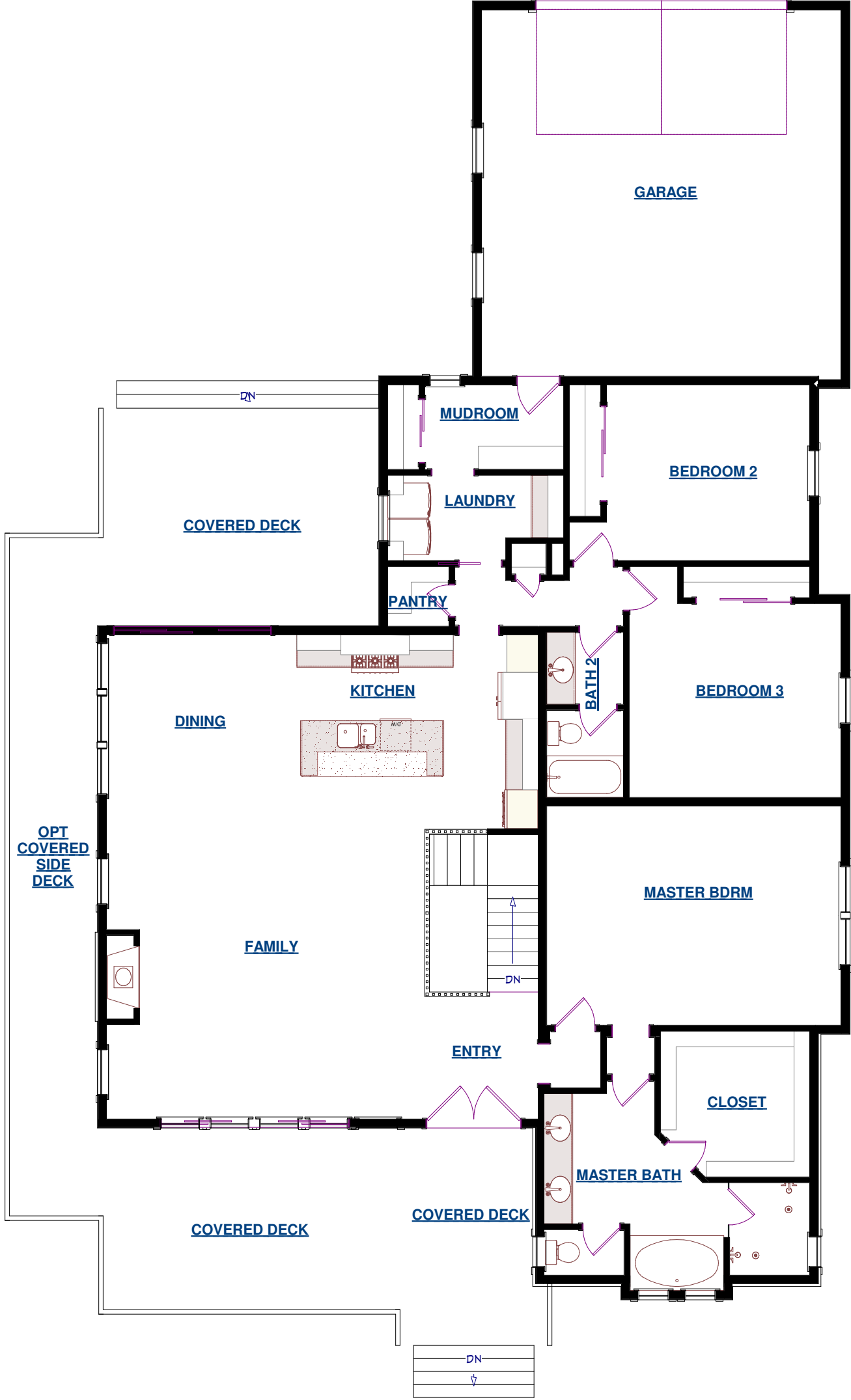
MAIN LEVEL FLOOR PLAN 2093 sq ft
