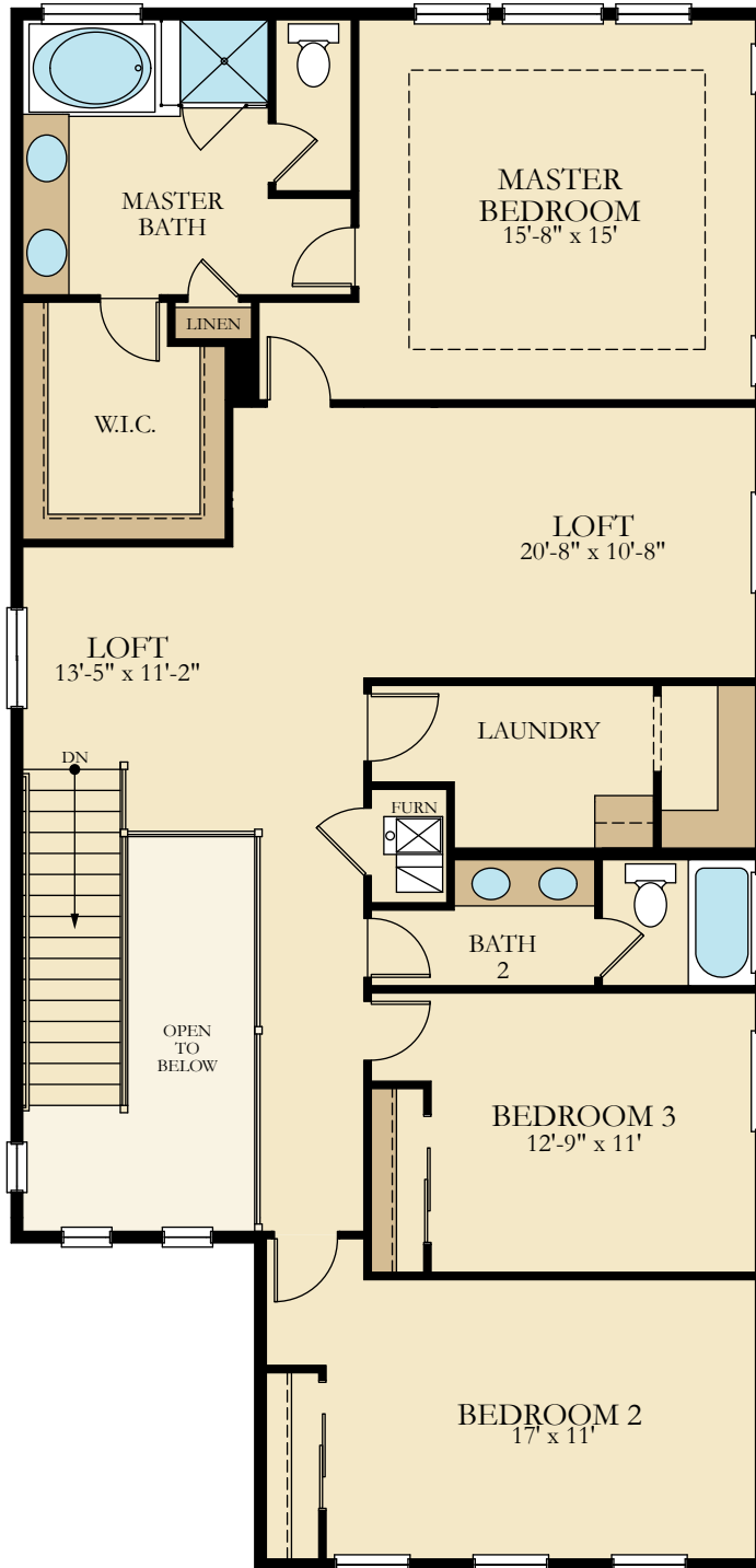
SECOND FLOOR
